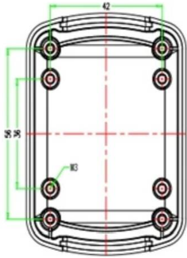
TOP ENCLOSURE INSIDE VIEW
