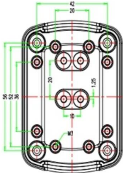
BOTTOM ENCLOSURE INSIDE VIEW
