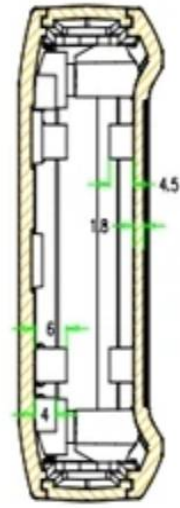
SEC B-B
