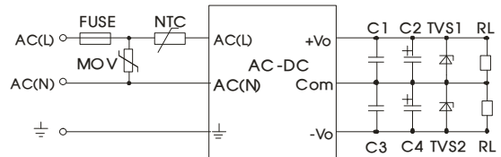
Fig. 2: LH20-10A series (Dual Output) typical application circuit
