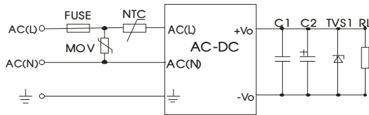
Fig. 1: LH20(25)-10B series (Single Output) Typical application circuit
