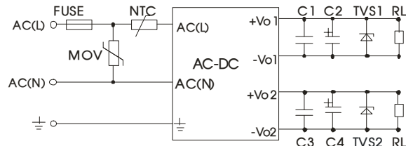
Fig. 4: LH20-10D series (Isolate Twin Output) typical application circuit
