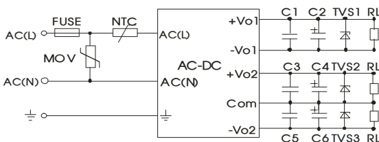
Fig. 3: LH20-10C series (Triple Output) typical application circuit
