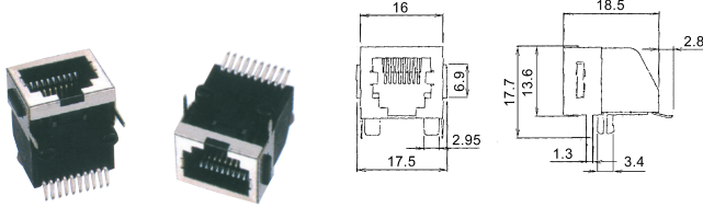
X98137 MODULAR SHIELDED JACK (8P8C) SMD TYPE
