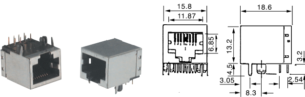
X98139SC MODULAR SHIELDED JACK (8P8C)
