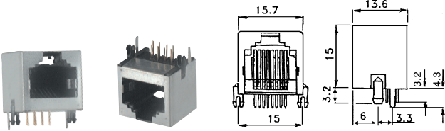
X98139SA MODULAR SHIELDED JACK (8P8C)
