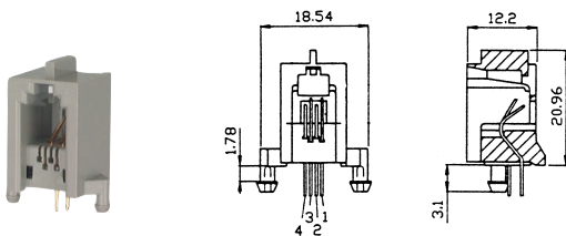
X98234 TELEPHONE JACK (623 TYPE 6P4C) X98236 TELEPHONE JACK (623 TYPE 6P6C)
