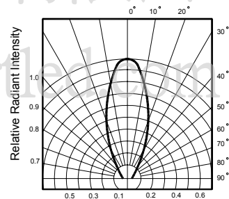
FIG.5 Radiant Diagram
