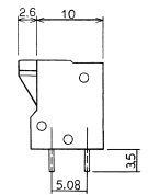
X97700A /B 5mm Terminal block
