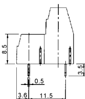
X97710A /B 5mm Terminal block
