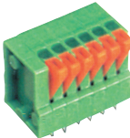
X97651A /B 2.54mm Terminal block
