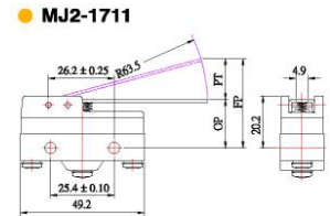
MJ2-1711 Micro switch, plastic body, IP67 MJ2-1711P Micro switch, phenolic body, IP67
