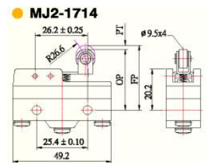
MJ2-1714 Micro switch, plastic body, IP67 MJ2-1714P Micro switch, phenolic body, IP67
