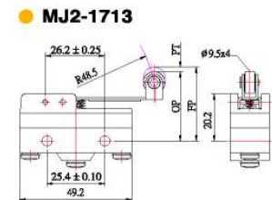
MJ2-1713 Micro switch, plastic body, IP67 MJ2-1713P Micro switch, phenolic body, IP67
