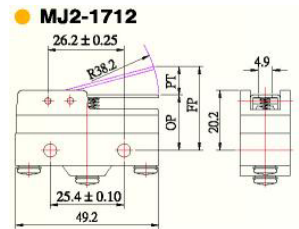
MJ2-1712 Micro switch, plastic body, IP67 MJ2-1712P Micro switch, phenolic body, IP67
